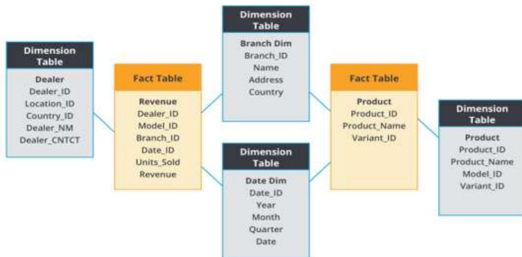
Example of Galaxy Schema
